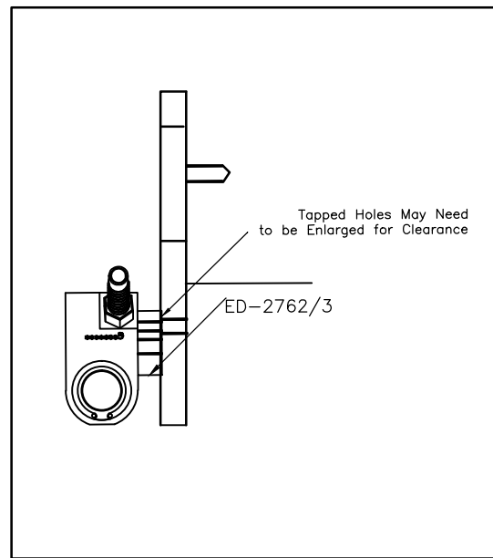
Spherosyn/SHG/DSG Series
