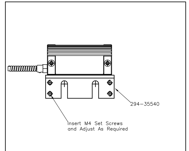
Spherosyn/SHG/DSG Series
