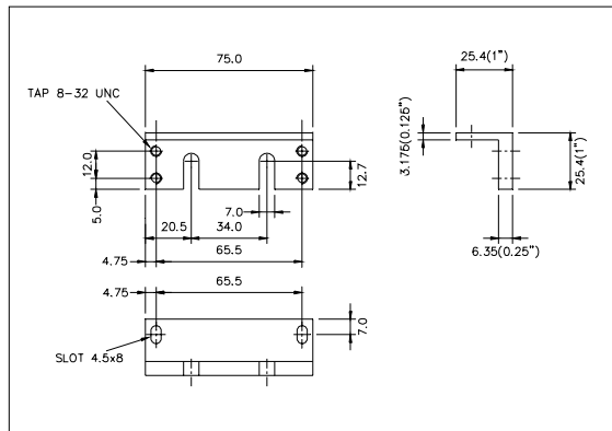
Part # 294-35260
