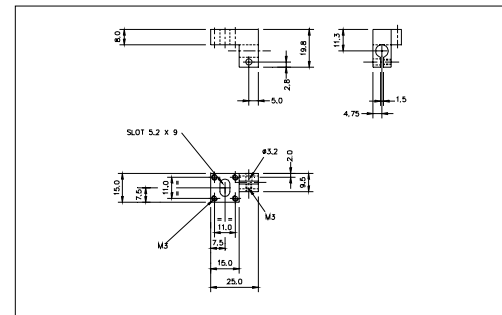
Single End Mount
