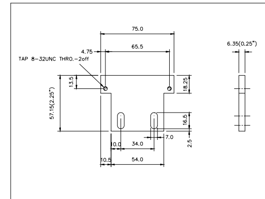
Part # 294-35270
