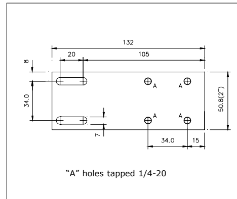
Part # 294-22510
