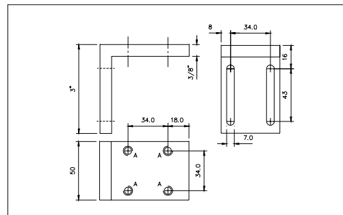
Part # 294-22530
